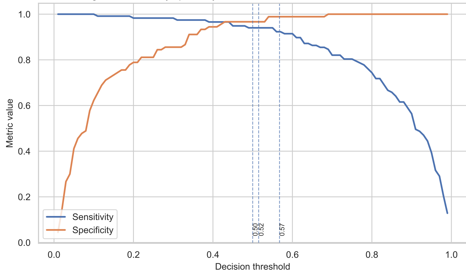
Figure 8. Sensitivity-specificity trade-off across thresholds — Random Forest
